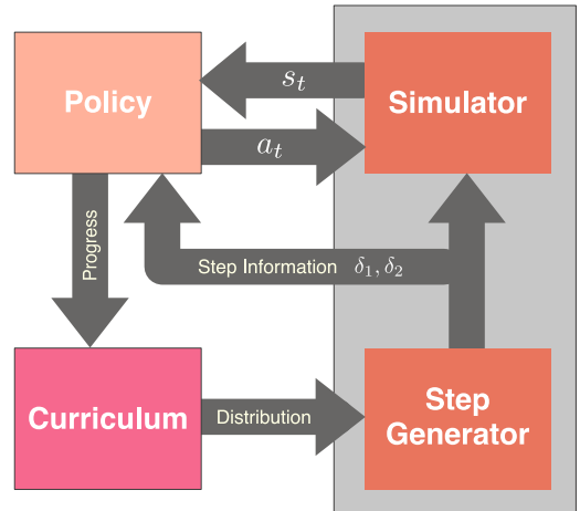
Figure 2: Overview of our curriculum learning system. The curriculum module improves learning efficiency by dynamically adjusting the terrain difficulty according to the progress of the policy.
