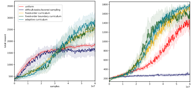
Figure 6: Learning curves for different sampling strategies, averaged over five runs. Left: Humanoid Right: Cassie.
