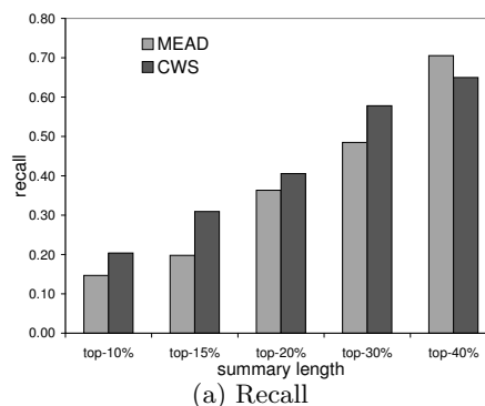
(a) Recall
