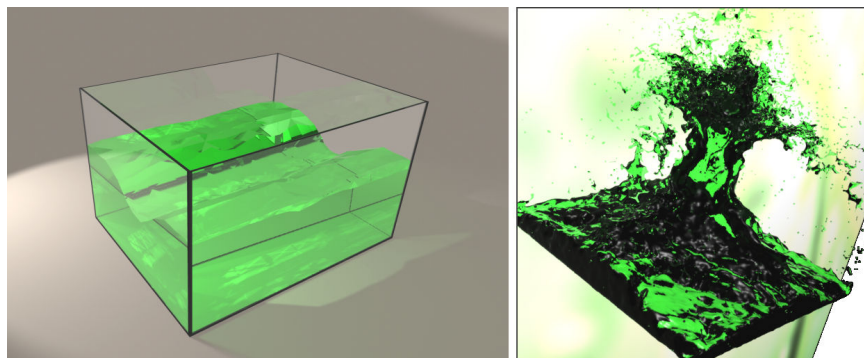
Figure 3.5: (Left) Isolation of fluid-air-boundary surface pairs. Through intersection and triangulation procedures the fluid-air, fluid-boundary and boundary-air surfaces were isolated, allowing interface-specific rendering parameters such as dielectric ratios to be applied to each surface pair. (Right) Another rendering of a transparent fluid surfaced using our algorithm.
