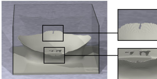
Figure 2.2: This image from Losasso et al. [38] shows unexpected mass loss (top right) as well as undesirable voxelization at the limits of the octree (top right and bottom right).
