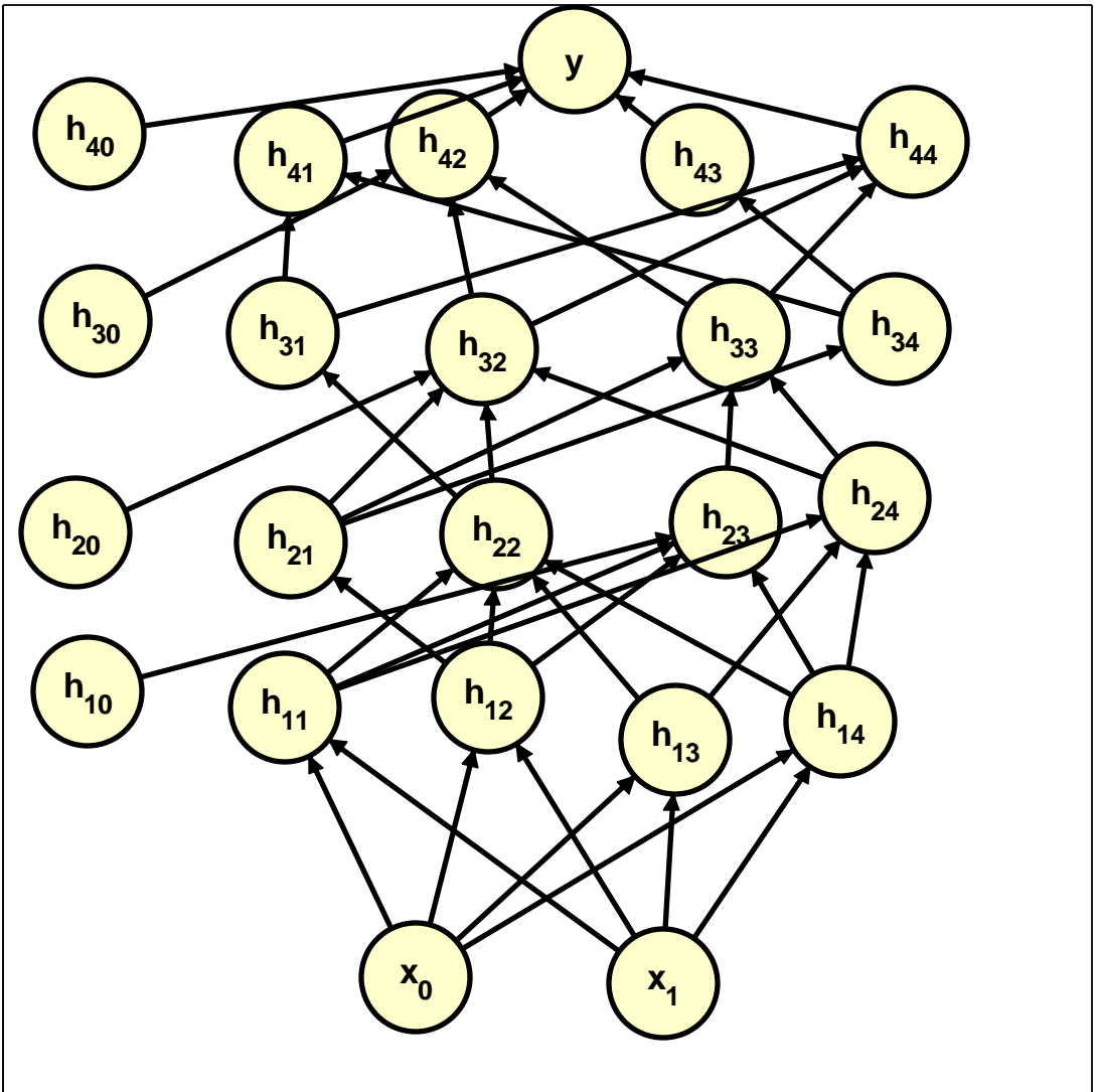
Neural Network
