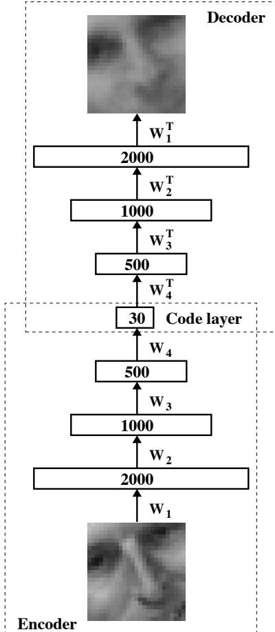
Unrolling
