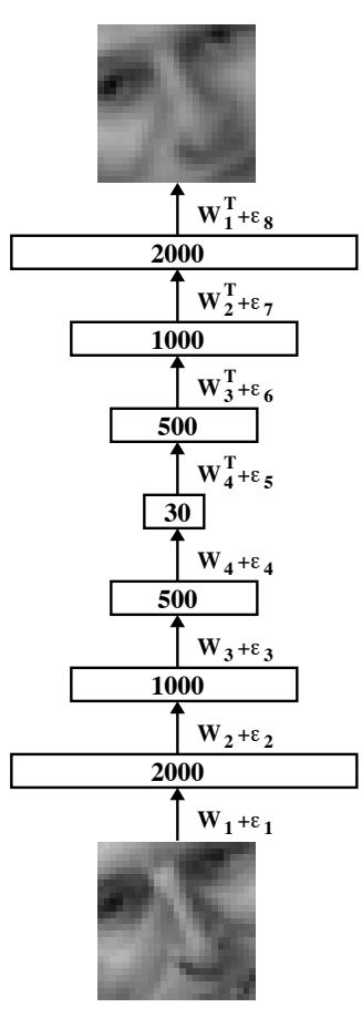
Fine-tuning
