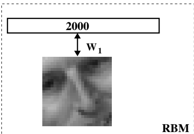
Pretraining
