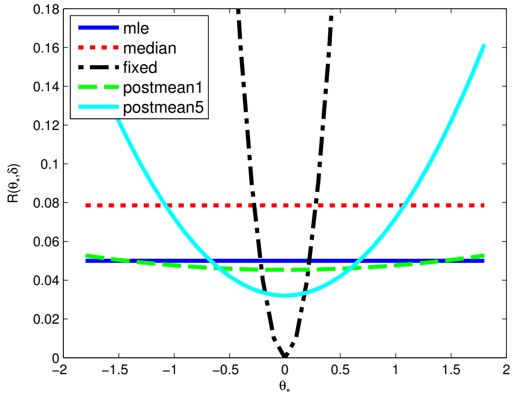
risk functions for n=20
