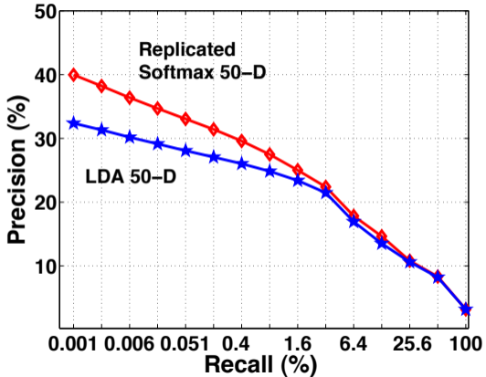
Reuters
