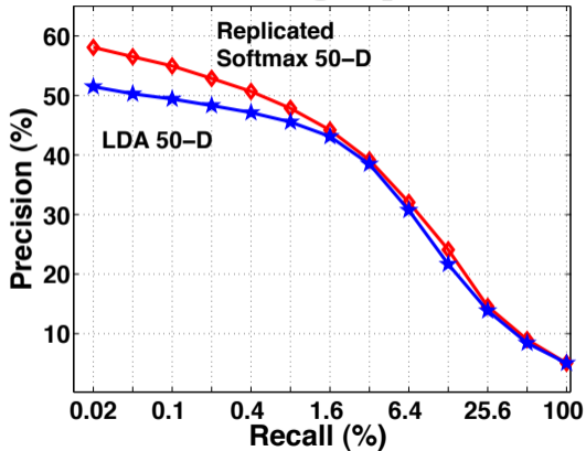
20-newsgroups
