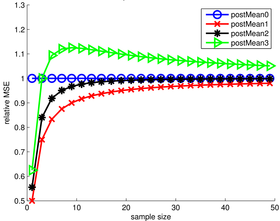
MSE of postmean / MSE of MLE
