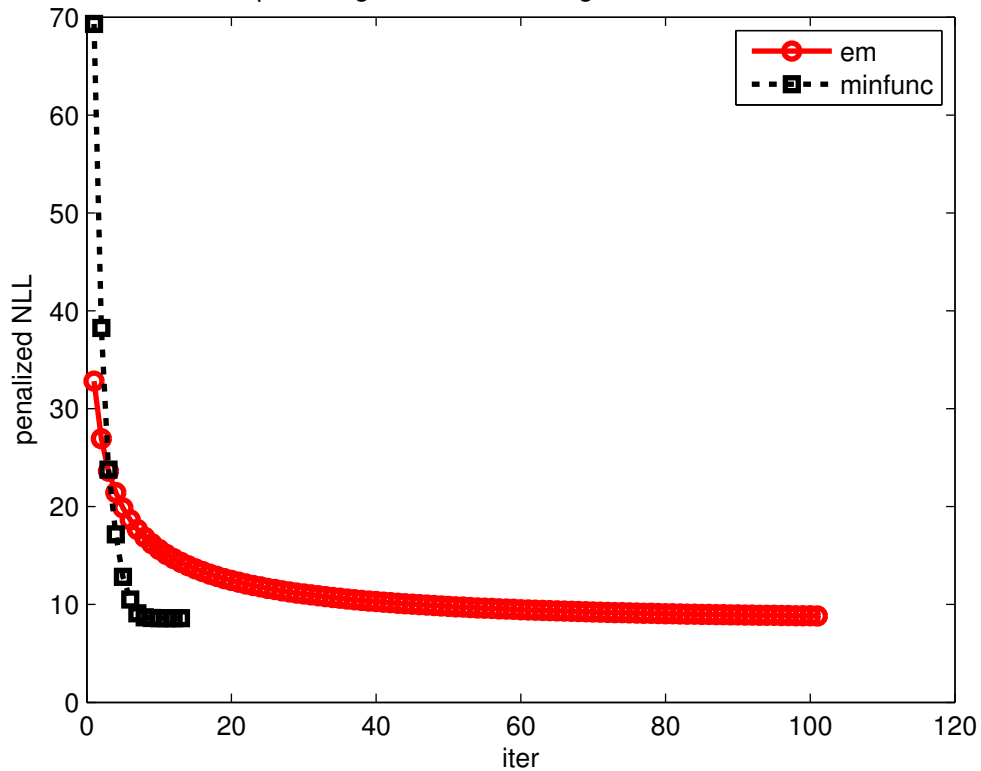
probit regression with L2 regularizer of 0.100
