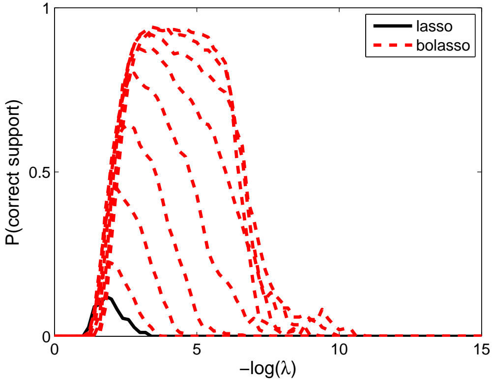
lasso vs bolasso on sign inconsistent data nbootstraps = [0,2,4,8,16,32,64,128,256]
