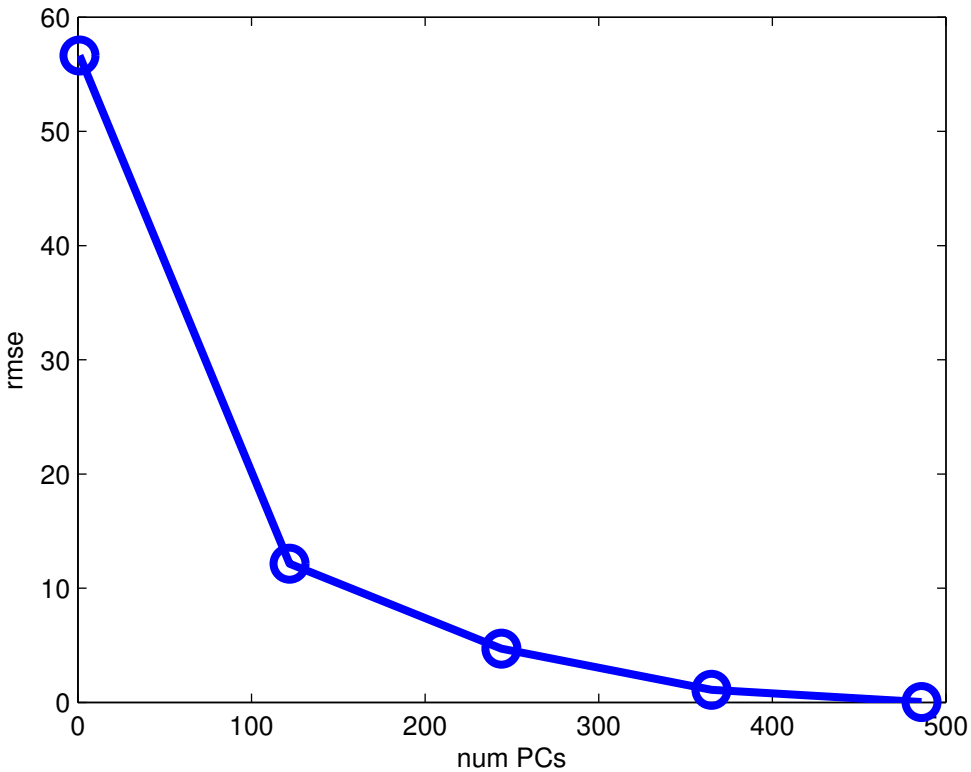
train set reconstruction error
