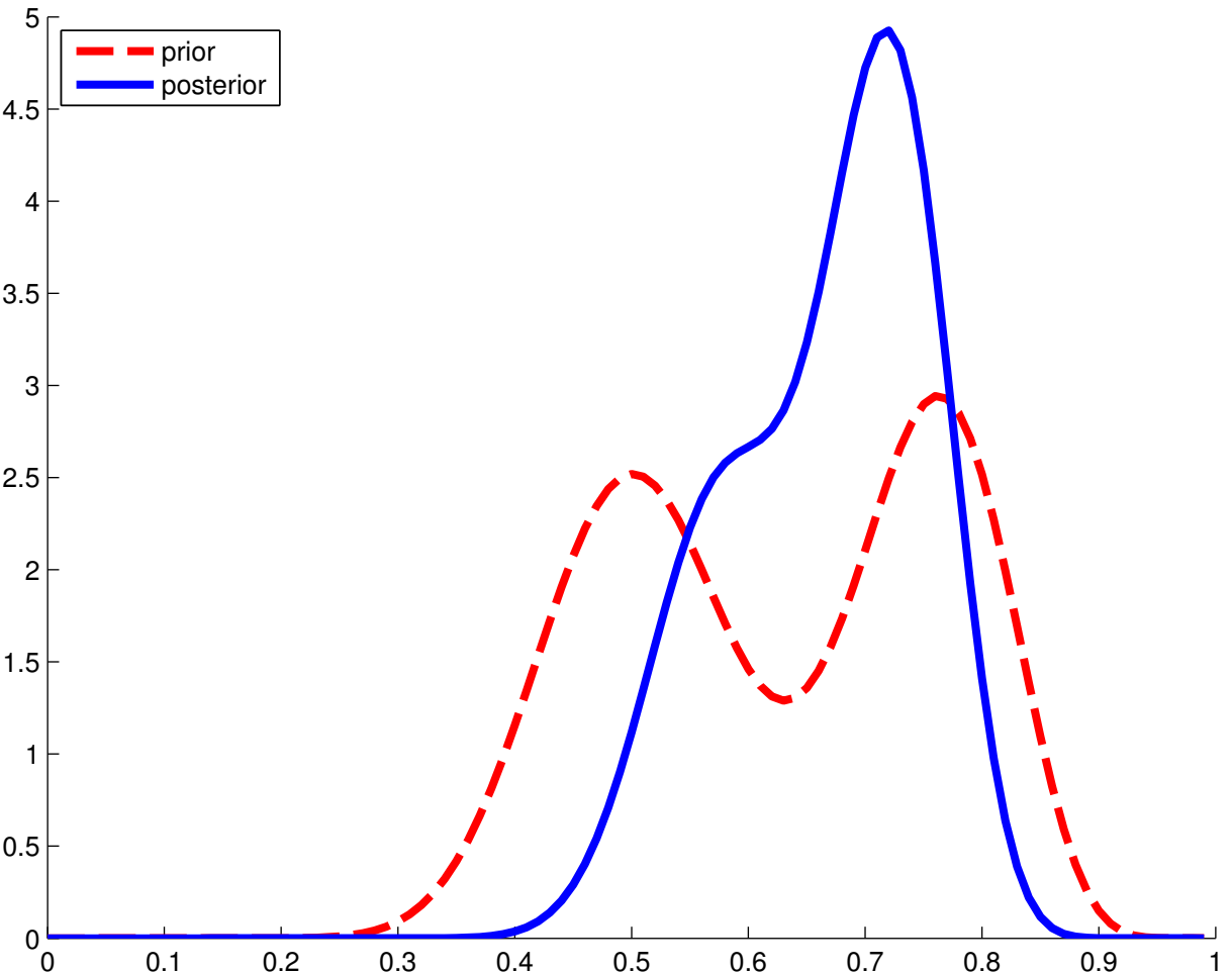
mixture of Beta distributions
