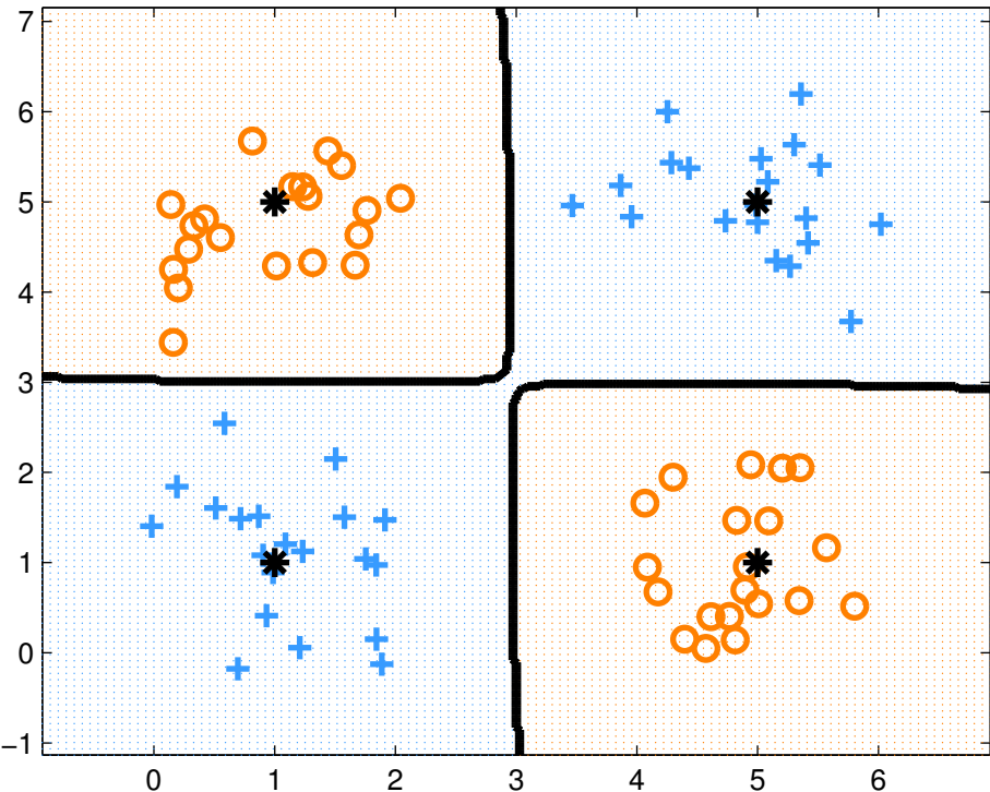
rbf prototypes
