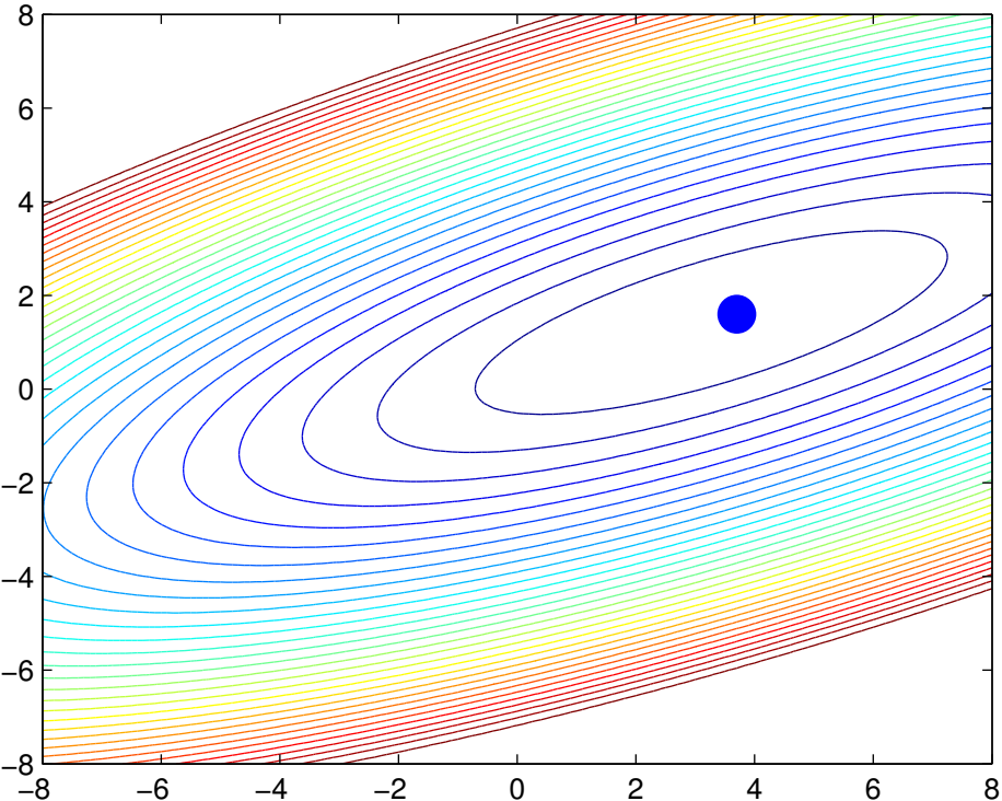
Laplace Approximation to Posterior
