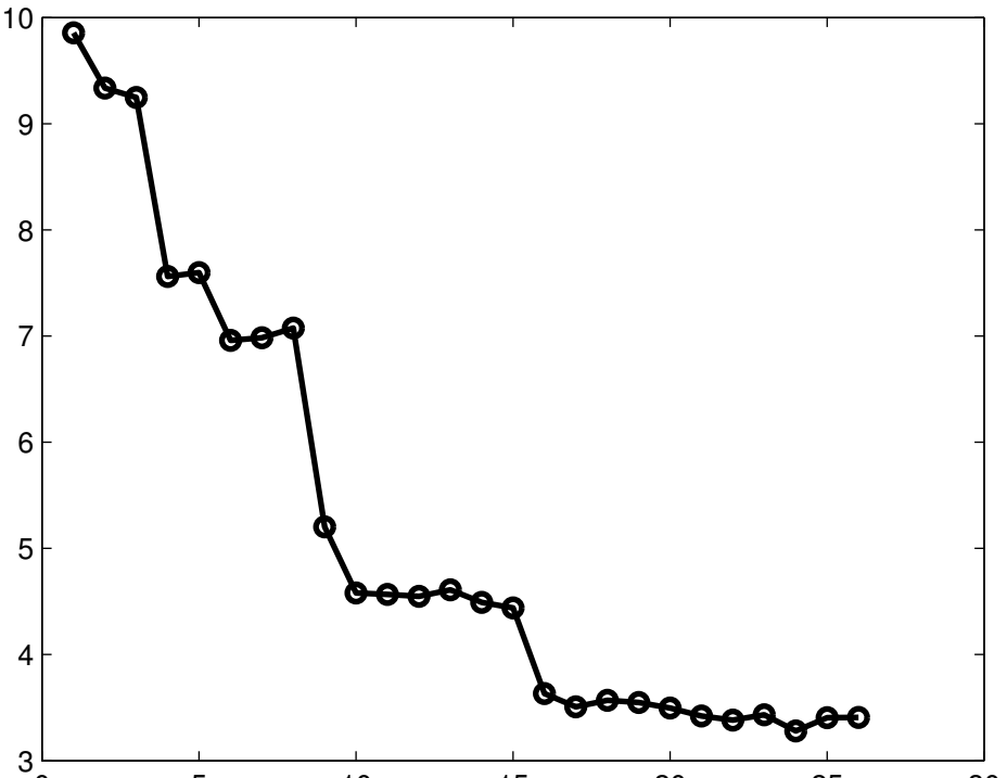
RSS vs iteration
