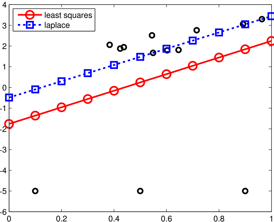
Linear data with noise and outliers
