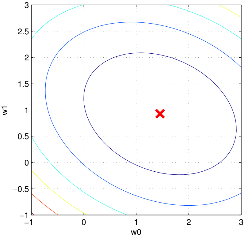
Sum of squares error contours for linear regression
