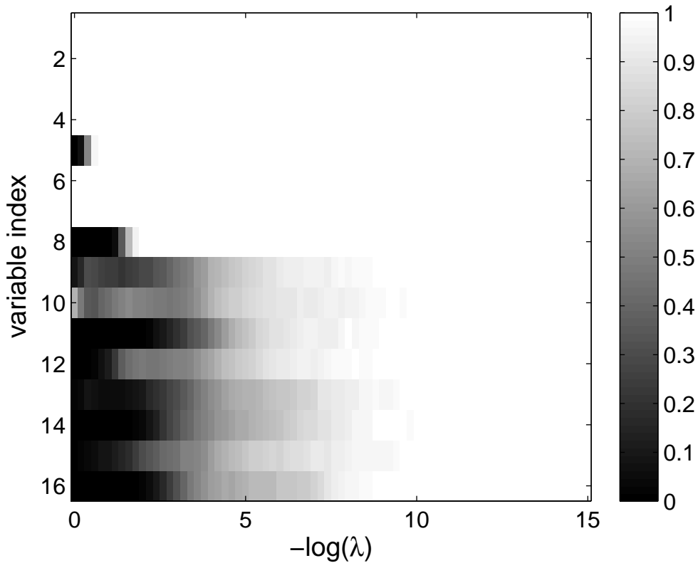
lasso on sign inconsistent data
