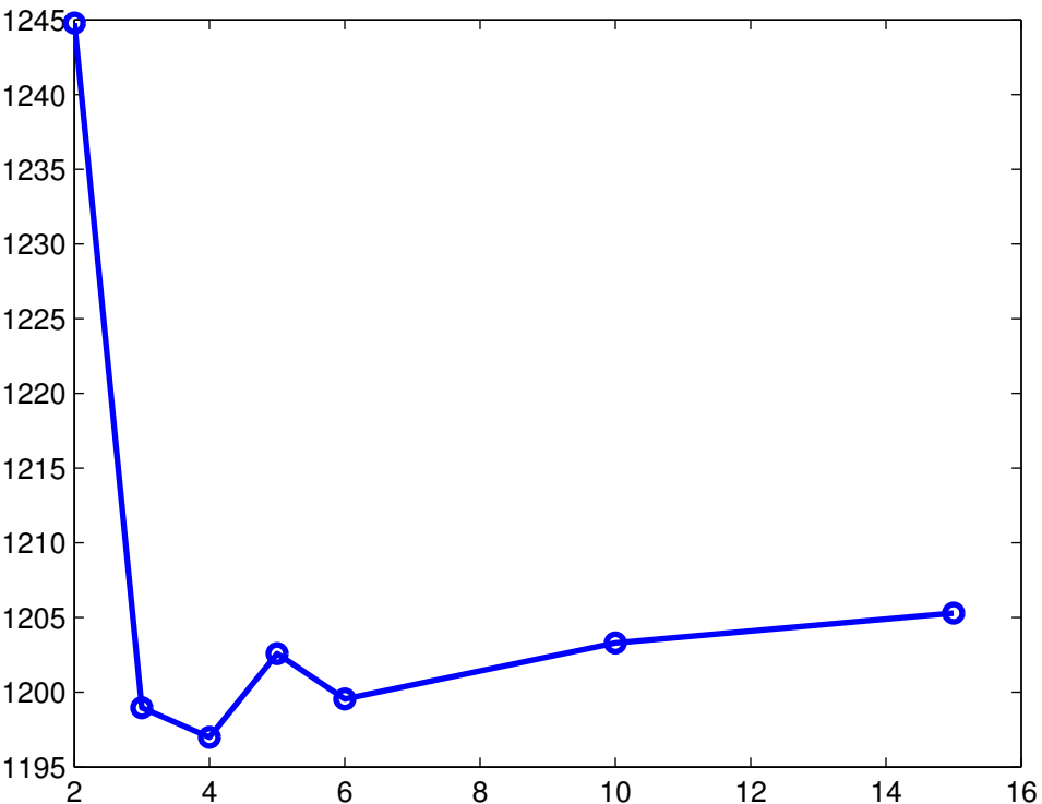
NLL on test set vs K for GMM
