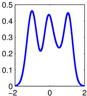
K=6, nll=1199.5574
