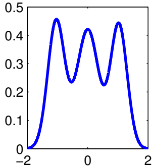
K=4, nll=1196.9937
