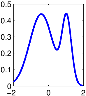
K=2, nll=1244.7882
