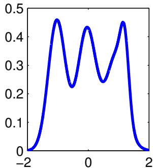
K=10, nll=1203.2931
