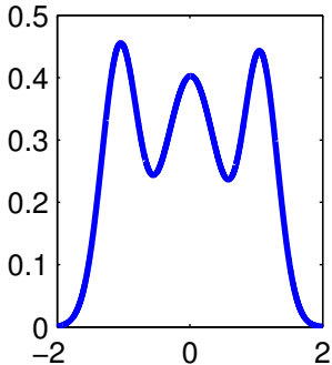
K=3, nll=1198.9738
