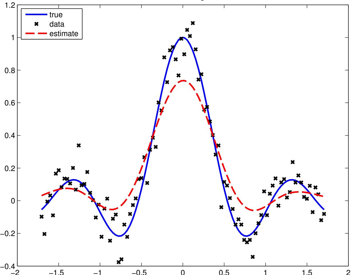
Gaussian kernel regression
