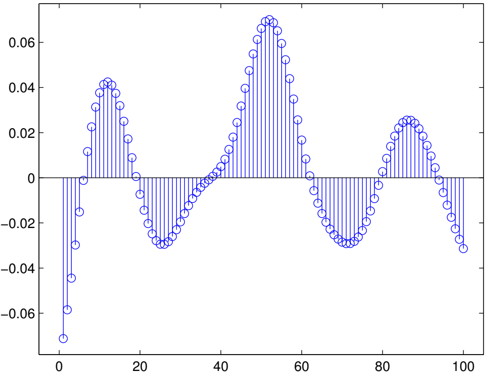
weights for linregL2
