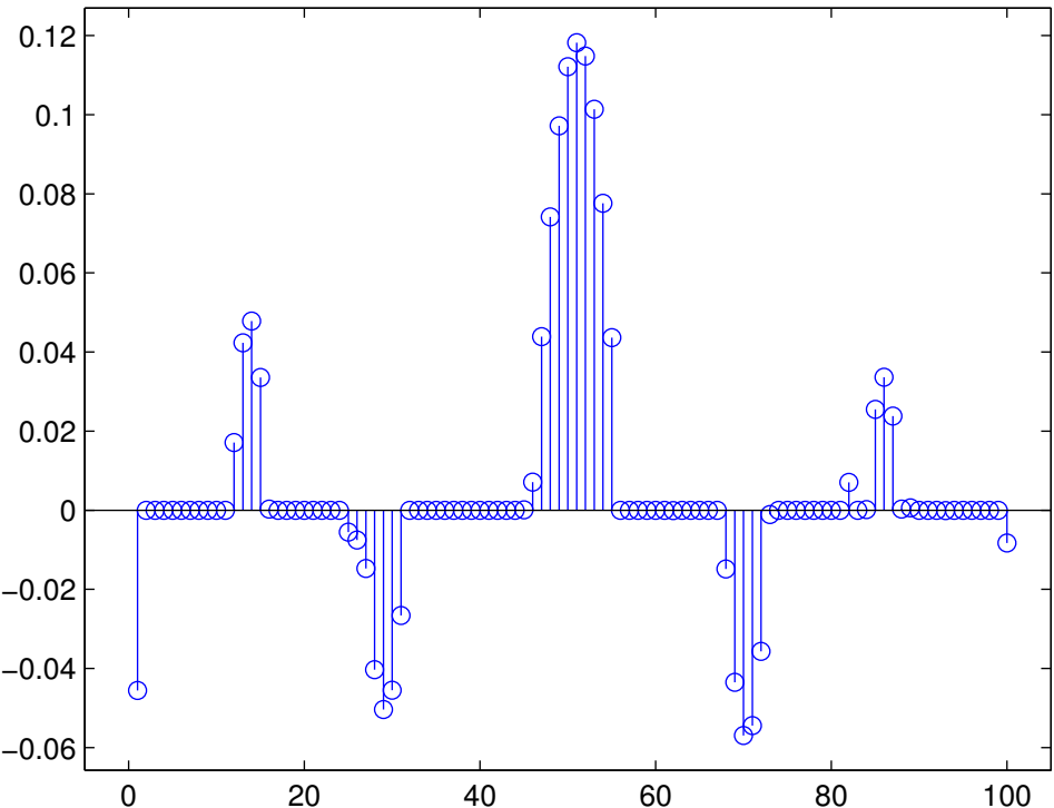
weights for linregL1
