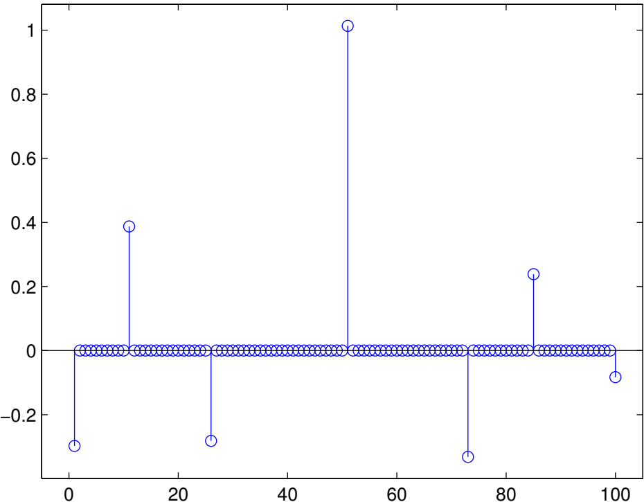
weights for RVM
