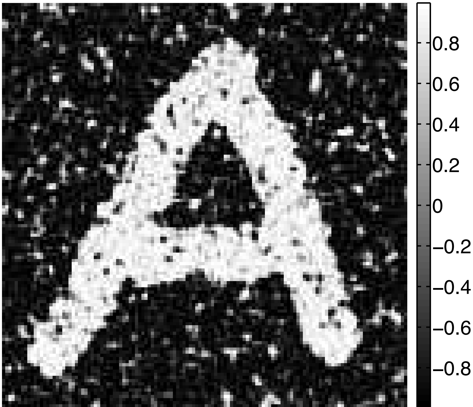
sample 3, meanfieldH
