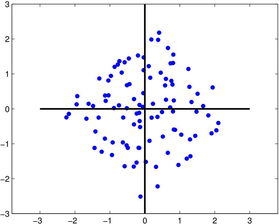
PCA applied to mixed data from uniform source
