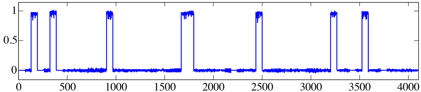
Block-Linf (debiased 1, \tau = 0.356 , MSE = 0.000425)
