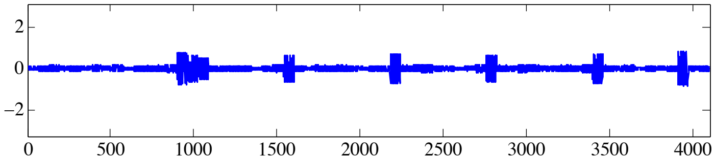
Block-Linf (debiased 1, \tau = 0.385 , \text{MSE} = 0.053 )
