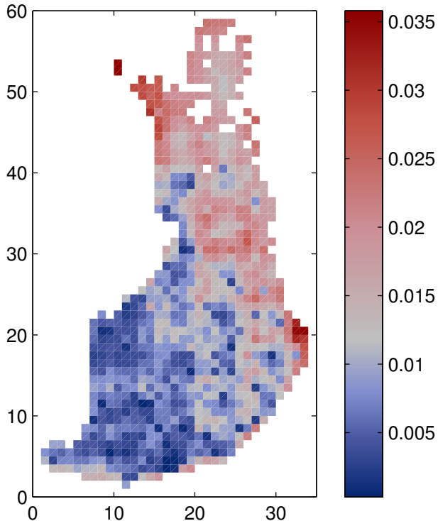
Posterior variance of the relative risk, FIC
