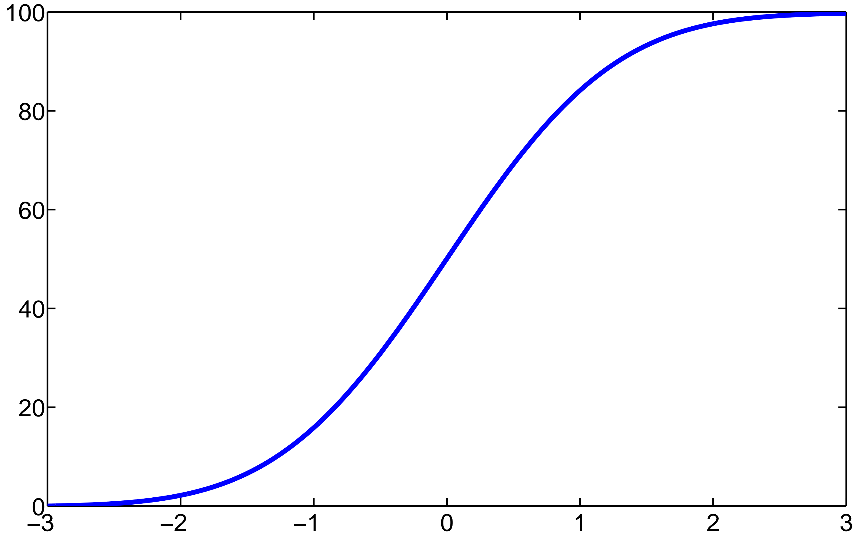
CDF
