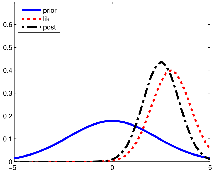
prior variance = 5.00
