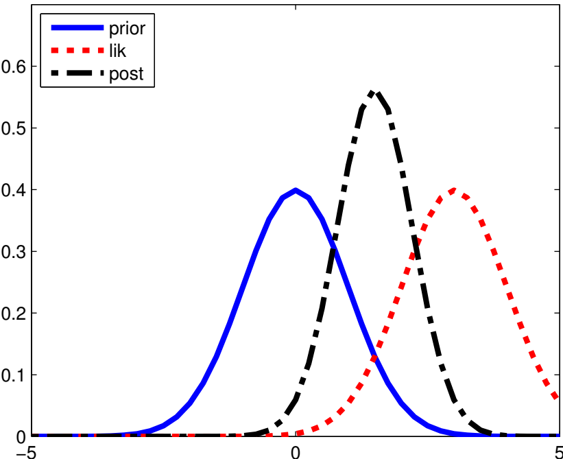
prior variance = 1.00
