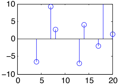
observed
