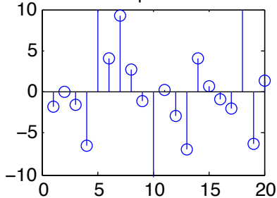
imputed
