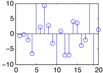
truth
