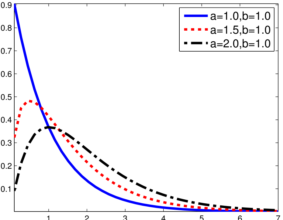
Gamma distributions
