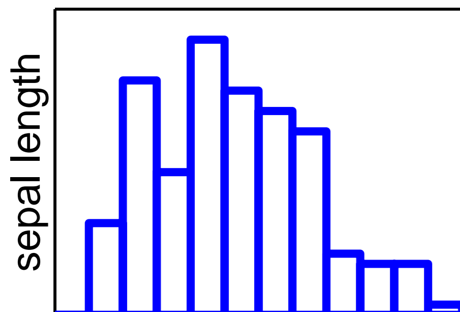
sepal length
