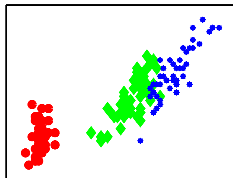
petal length
