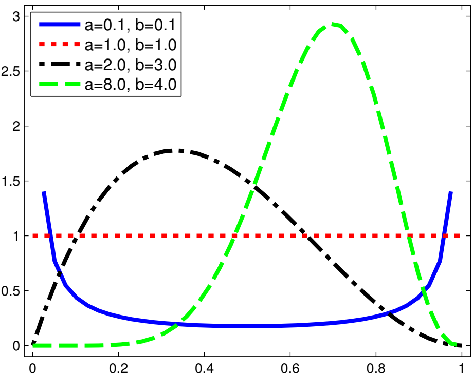
beta distributions
