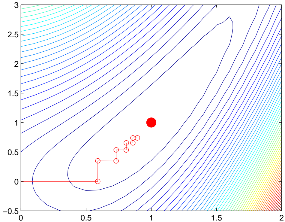
exact line searching 1
