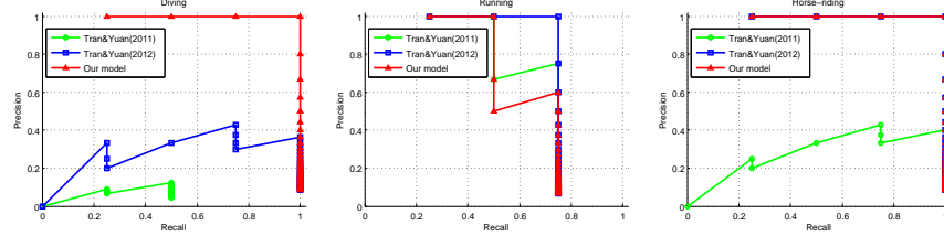
Figure 2: Precision-Recall curves for localization: We compare our model ( Region+Context with K=1 latent region) to the method from [18] and [19].
