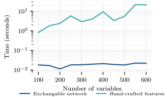
Figure 2: Average running times per instance as size varies for the exchangeable architecture and hand-engineered features. Note the log scale on the y-axis.
