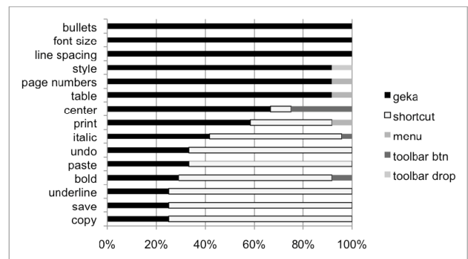
Figure 6: Percentage of command executions using each method in the method choice phase of the experiment ( N=12 ).
