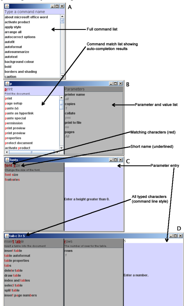
Figure 3: GEKA prototype graphical feedback showing four distinct phases of interaction. Part A is before anything has been typed, B shows command name selection, C shows inputting a parameter for a command with only one parameter, and D shows inputting a parameter for a command with multiple parameters.
