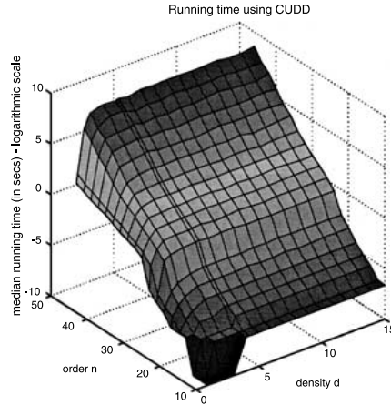
Figure 8. CUDD – 3-D Plot of median running time.
