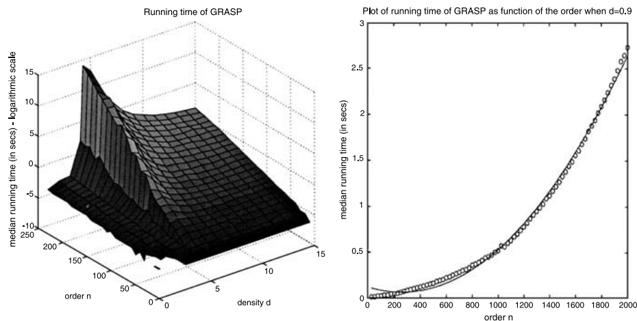
Figure 1. GRASP – (left) 3-D Plot of median running time, and (right) median running time for density 0.9 as a function of the order of the instances. A quadratic function fits these points better (with an r^2 > 0.98 ) than an exponential function.
