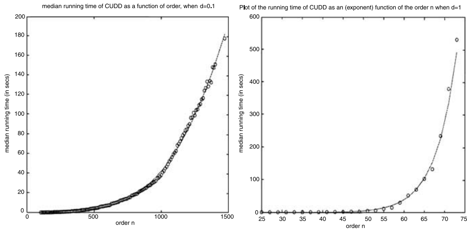
Figure 9. CUDD – median running time for density 0.1 (left) and for density 1 (right) as a cubic and an exponential respectively function of the order of the instances.
