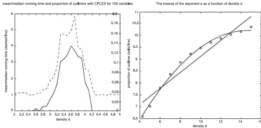
Figure 7. CPLEX – (left) Ratio of mean-to-median running time and proportion of outliers, and (right) the exponent 1/\alpha of median running time as a function of density.
