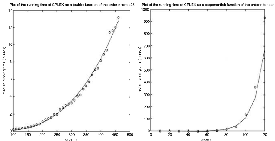
Figure 6. CPLEX – median running time for density 2.5 (left) and density 4 (right) as a cubic and exponential function respectively, of the order of the instances.
