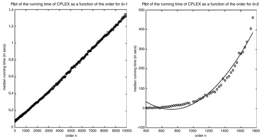
Figure 5. CPLEX – median running time for density 1 (left) and density 2 (right) as a function of the order of the instances.
