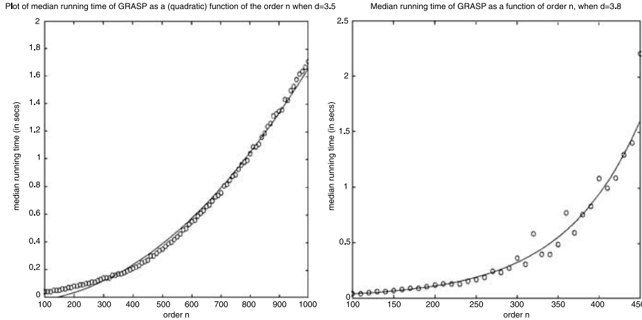
Figure 2. GRASP – median running time for density 3.5 (left) and density 3.8 (right) as a function of the order of the instances. At density 3.5, the best fit curve is quadratic in the order, while at 3.8, the best fit curve is exponential in the order.
