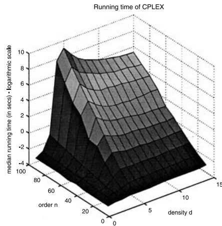
Figure 4. CPLEX – 3-D Plot of median running time.
