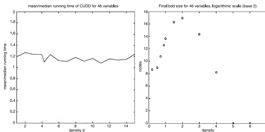
Figure 10. CUDD – (left) Ratio of mean-to-median running time and (right) median ROBDD size as a function of density.
