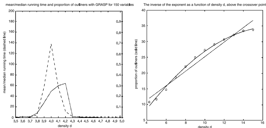
Figure 3. GRASP – (left) Ratio of mean-to-median running time and the proportion of outliers, and (right) the exponent 1/\alpha of median running time as a function of density.
