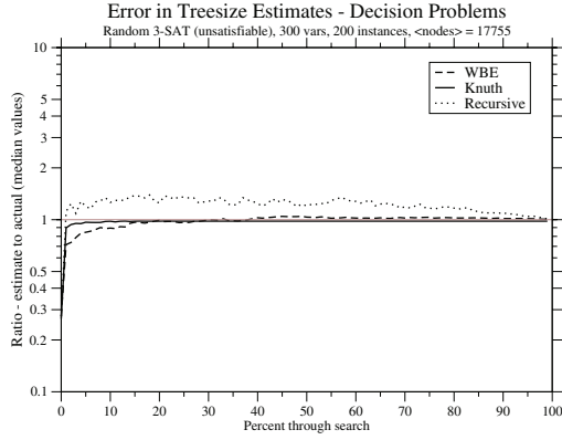
Figure 3: Treesize estimates, unsatisfiable decision problems “3-unsat”
