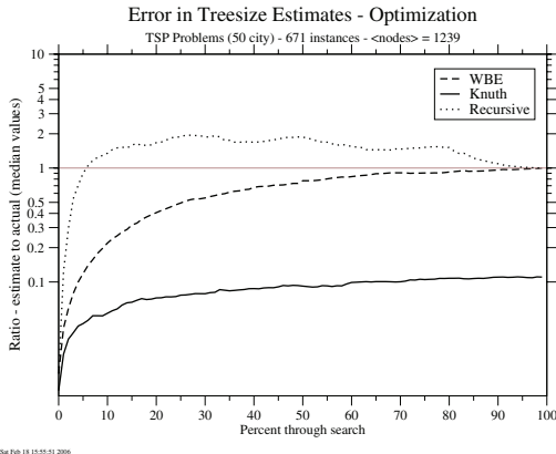
Figure 6: Treesize estimates, optimization problems “tsp”
