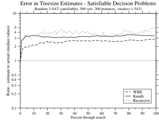
Figure 7: Treesize estimates, satisfiable decision problems “3-sat”
