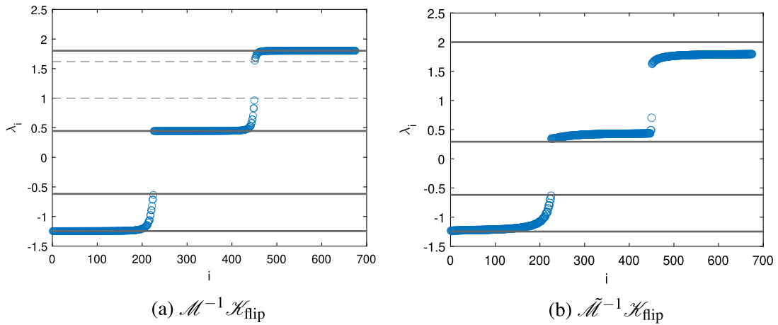
FIG. 3. Eigenvalue plots for reordered distributed Poisson control matrix \mathcal{K}_{\text{flip}} , with exact preconditioner \mathcal{M} (left) and approximate preconditioner \tilde{\mathcal{M}} (right). Eigenvalues are shown by the circles; eigenvalue bounds (from Theorem 3.2 on left and Corollary 4.1 on right) are shown by lines.
