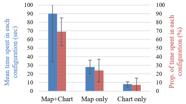
Figure 3: Time spent in each visualization configuration.
