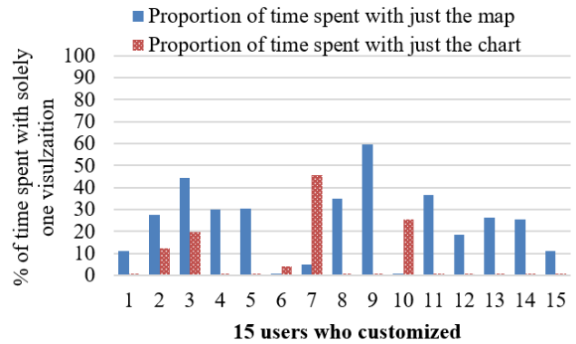
Figure 4: Prop. of time spent in each visualization configuration by the 15 users who customized.
