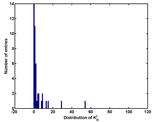
(b) \mathcal{K}_H^j distribution ( \mathcal{K}_H^j \leq 50 )
