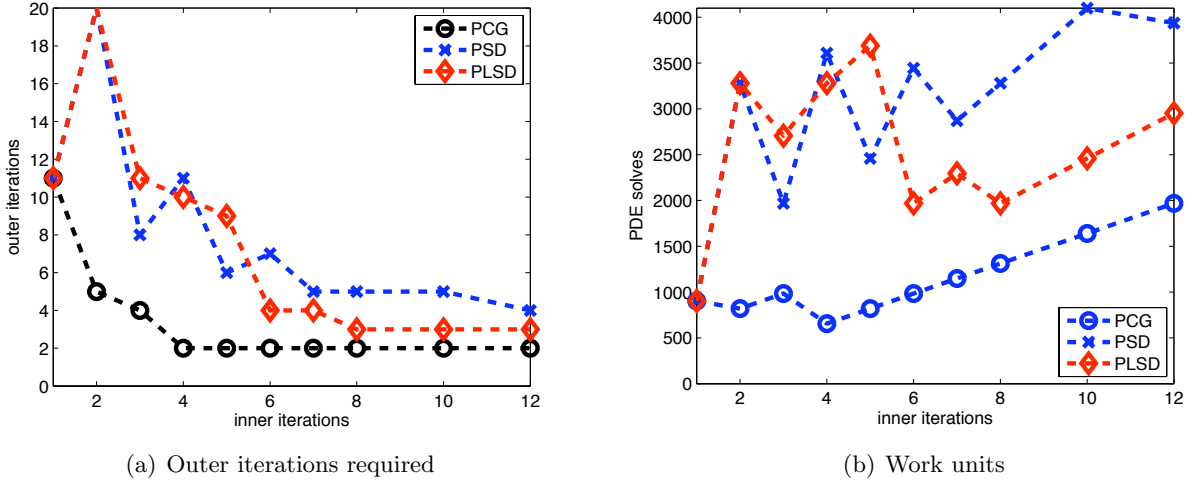
Figure 5: Inner iteration counts and number of PDE solves for the shape reconstruction problem of [12]. For iters_{in} = 1 all three methods coincide.
