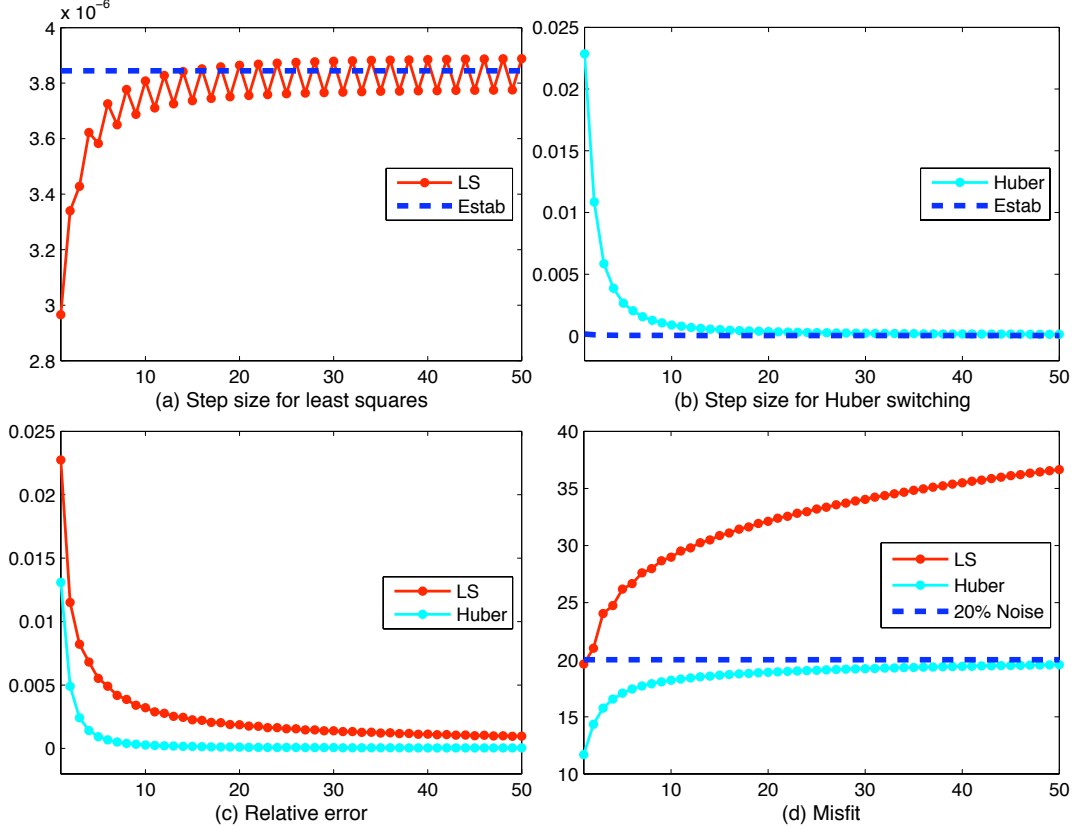
Figure 3: Discrete dynamics for the test problem Cameraman in Figure 4(a) with 20% white noise added. Two regularizations, LS ( \gamma large) and Huber switching ( \gamma by (18)), are compared. The horizontal axis displays iteration numbers.
