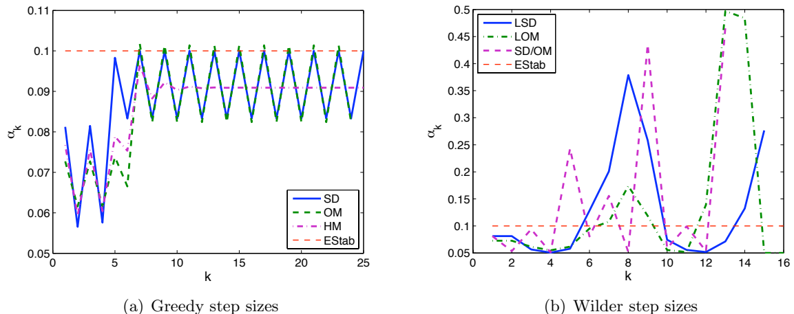
Figure 1: Step size dynamics for A = \text{diag}(20, 10, 2, 1) . (a) The greedy strategies produce orderly dynamical systems which have a steady state or are two-periodic. Forward Euler absolute stability limit, depicted here as ‘EStab’, therefore decrees slow convergence. (b) When this pattern is broken a faster convergence to steady state results.
