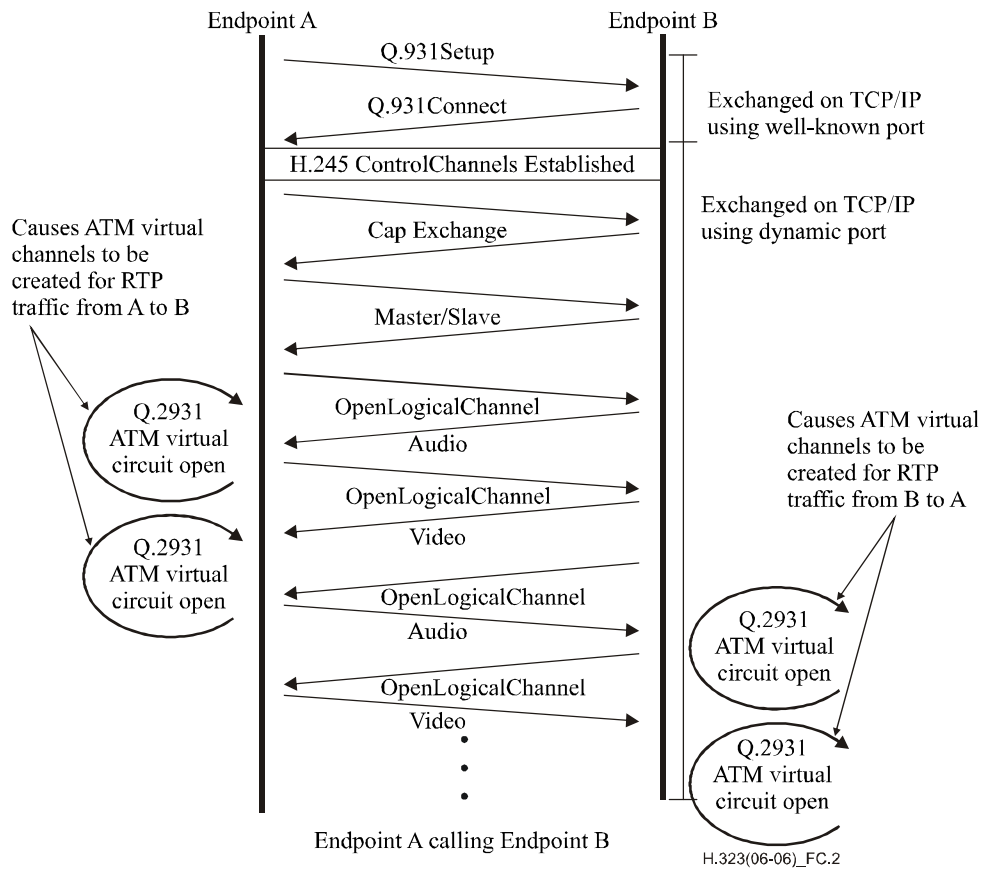
Figure C.2 – H.323 call establishment showing ATM effect – ATM VCs used unidirectionally
