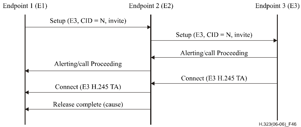
Figure 46 – Non-MC invite signalling
