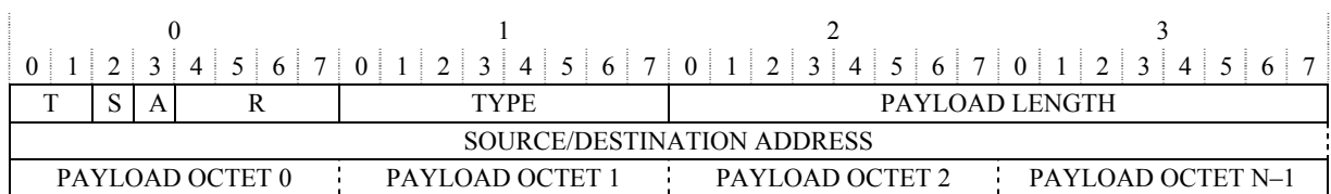
Figure E.17 – Extended-3 payload format
