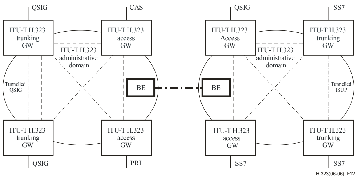
Figure 12 – Relationship of H.323, SCN and H.248 gateways
