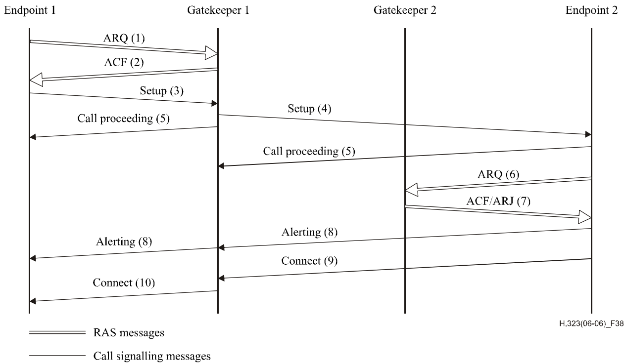
Figure 38 – Both endpoints registered – Routed/direct call signalling
