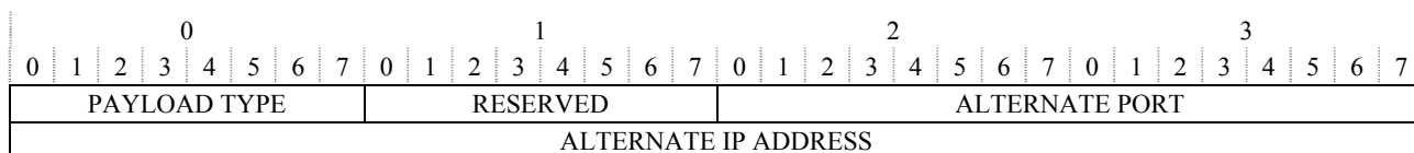
Figure E.10 – Nack reason 1 structure
