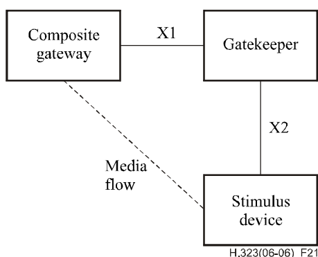
Figure 21 – Composite gateway and Annex L device
