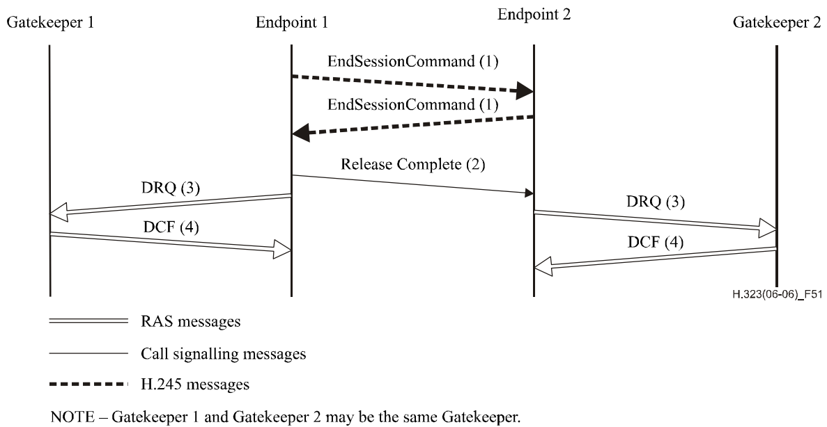
Figure 51 – Endpoint initiated call clearing (Procedure B)
