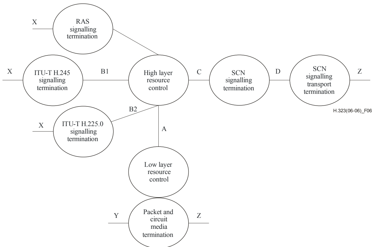
Figure 6 – Functional architecture of the decomposed gateway
