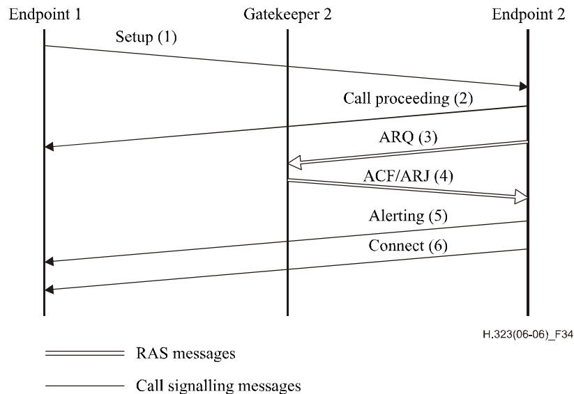
Figure 34 – Only called endpoint registered – Direct call signalling
