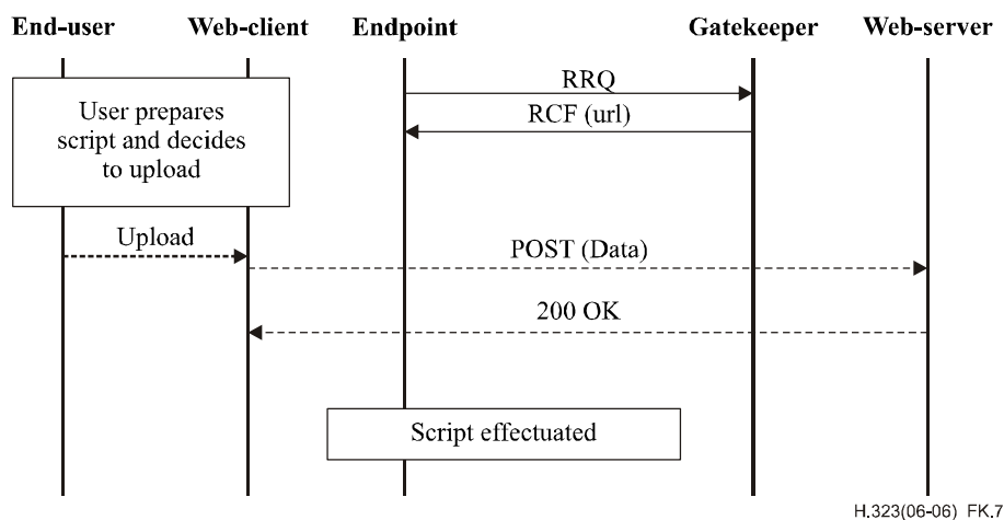
Figure K.7 – Non-call-related service control, script upload
