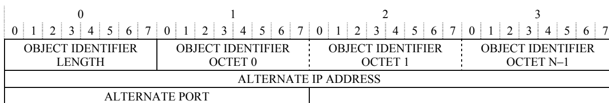
Figure E.11 – Nack reason 2 structure
