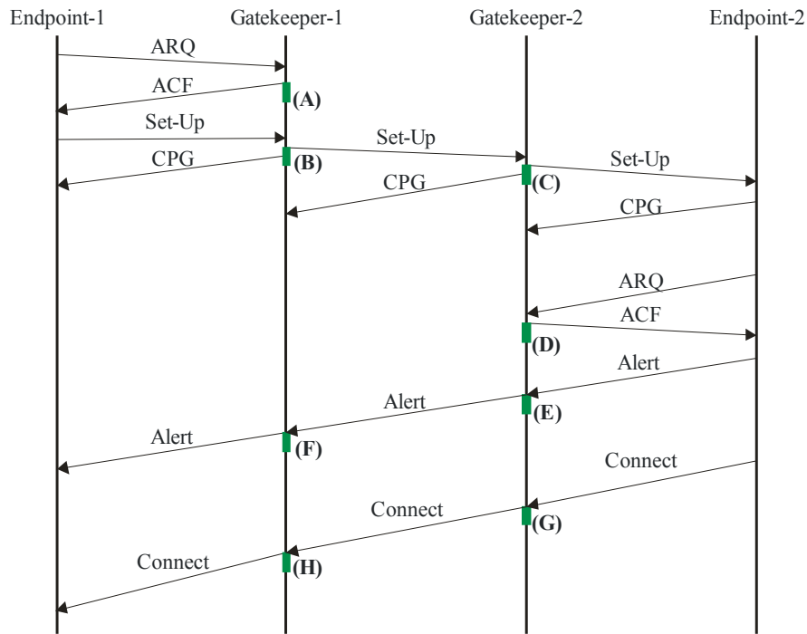
Figure VII.2 – Example H.323 call
