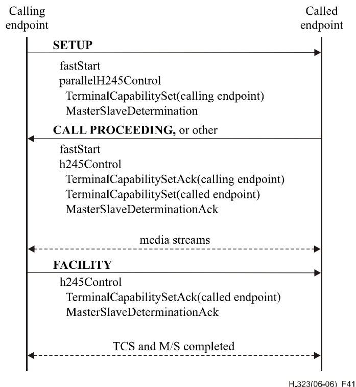
Figure 41 – Successful initiation of ITU-T H.245 in parallel with fast connect
