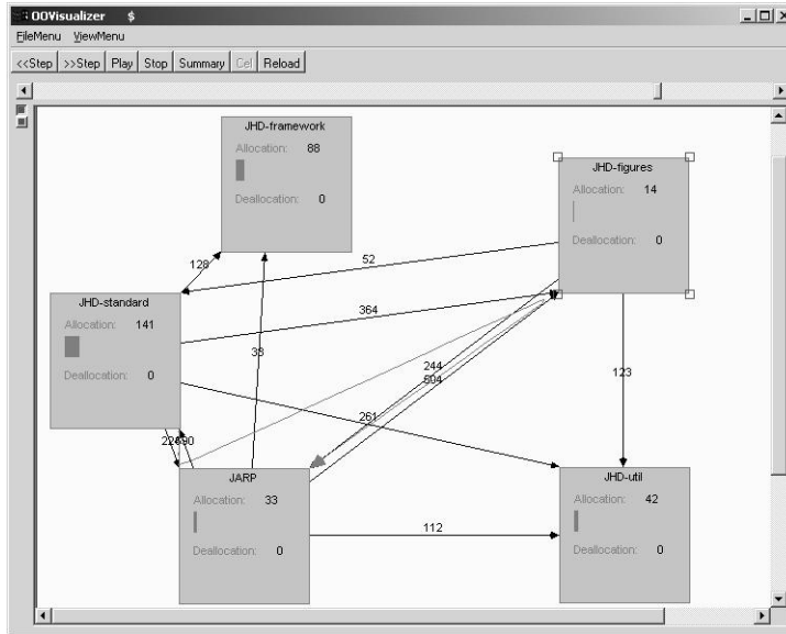
Figure 1. AVID with JARP Example Loaded
