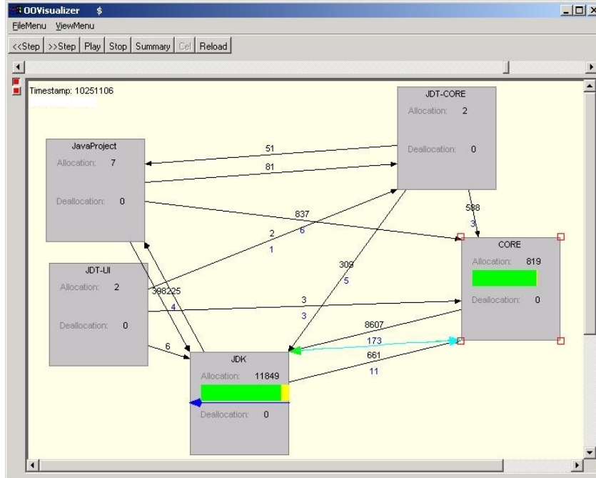
Figure 2. AVID with Trace from Unoptimized Filesystem Problem
