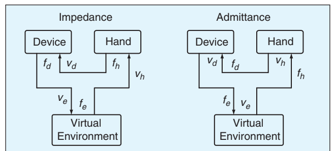
Figure 7. Abstracted mechanical circuits.
