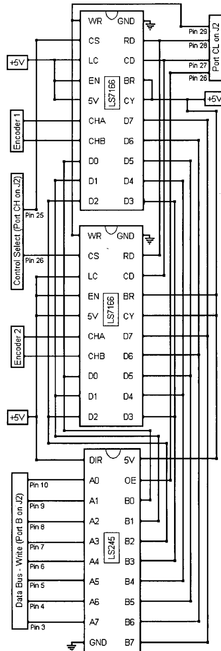
Figure 31 Encoder-decoder Circuit
