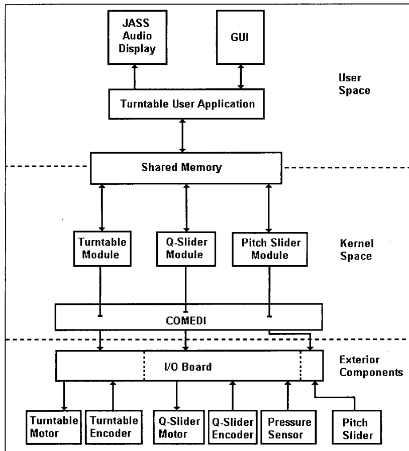
Figure 26 Software Component Schematic
