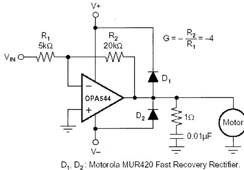
Figure 32 Amplifier for Q-slider Motor
