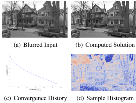
Figure 10. Convergence history of method down to e_d < 4 \times 10^{-9} for anisotropic TV regularizer with weight \lambda = 10^{-3} . Note that each Stochastic Deconvolution iteration has an approximately equal computational cost to one gradient-descent step using image-space convolutions but is able to focus sampling effort near details, as shown in the sampling histogram.
